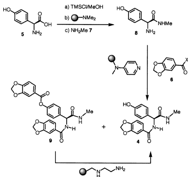
Scheme 2. Initial synthetic pathway. Preparation of fragment 4.
