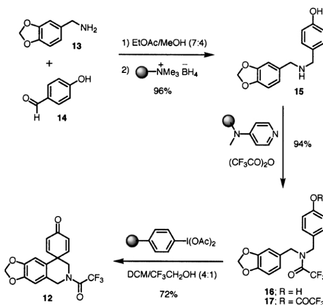
Scheme 4. Model compound preparation using solid-supported reagents.
