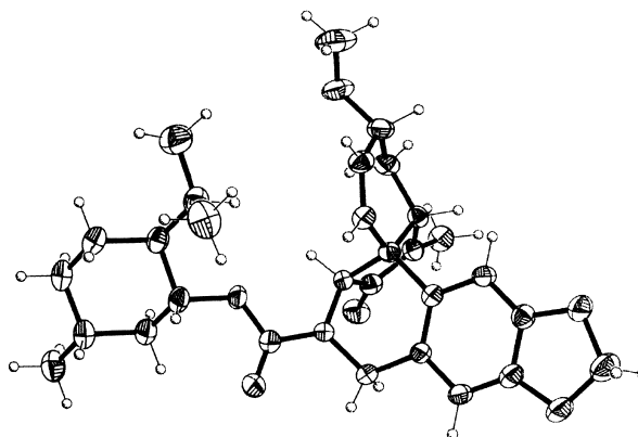
Figure 4. The X-ray crystal structure of the derivative 50 .
